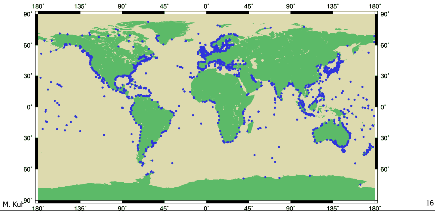
Distribution of PSMSL Stations
