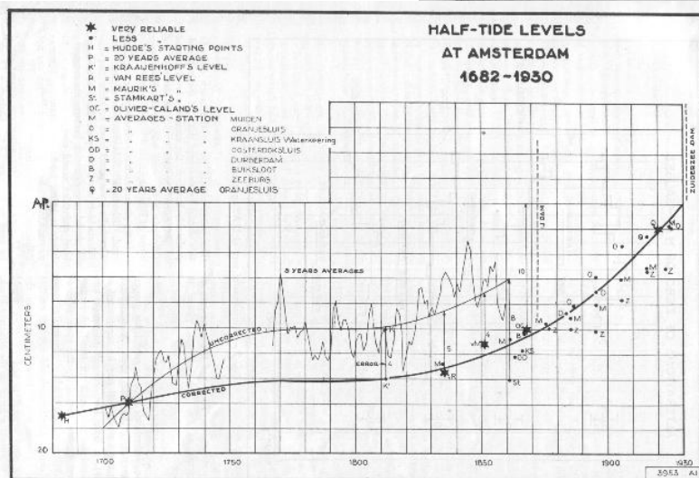
Fig. 1 — Half-tide levels at Amsterdam, 1682—1930.
